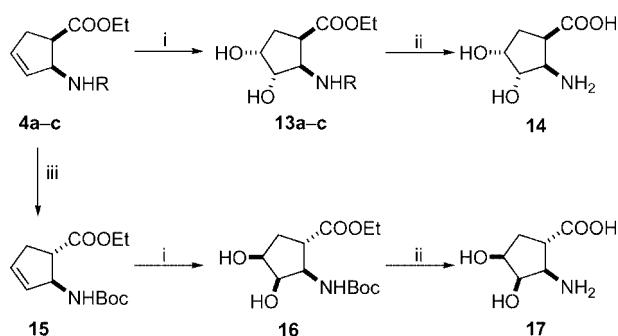
Scheme 3. Reagents and conditions: (i) 2.0 wt.-% solution of OsO 4 in t BuOH, NMO, acetone, 4 h, room temp.; R = Ac: 47%; R = Boc: 56%; R = Z: 58%; (ii) R = Ac: 20% HCl/H 2 O, Δ T , 48 h; R = Boc: 10% HCl/H 2 O, 24 h, room temp.; R = Z: 5% Pd/C, H 2 , EtOH, 12 h, room temp.; 20% HCl/H 2 O, Δ T , 24 h, 35–37%; (iii) NaOEt, EtOH, 24 h, room temp., 51%.
