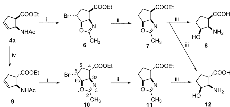
Scheme 2. Reagents and conditions: (i) NBS, CH 2 Cl 2 , 3 h, room temp., 71–86%; (ii) Bu 3 SnH, CH 2 Cl 2 , Ar, 20 h, \Delta T, 63–65%; (iii) 20% HCl/H 2 O, 24 h, \Delta T, 22–67%; (iv) NaOEt, EtOH, 24 h, room temp., 37%.
